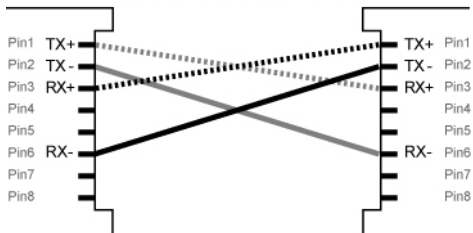
Cross-Over Cable Wiring
