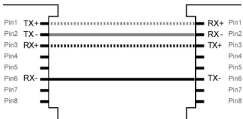
Straight Through Cable Wiring
